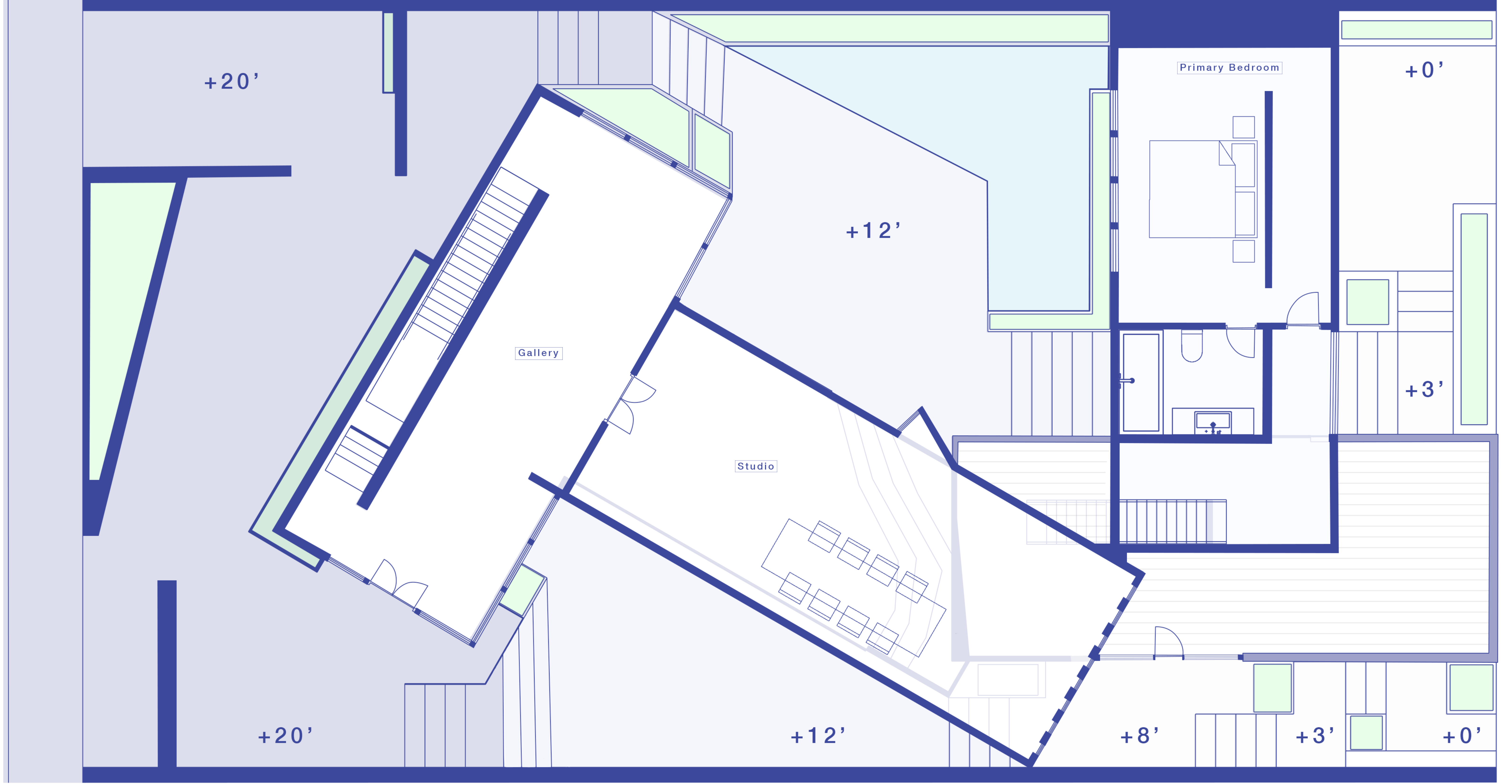
Floorplan Scale - 1/4"=1'
